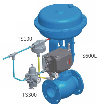
Single actuator
